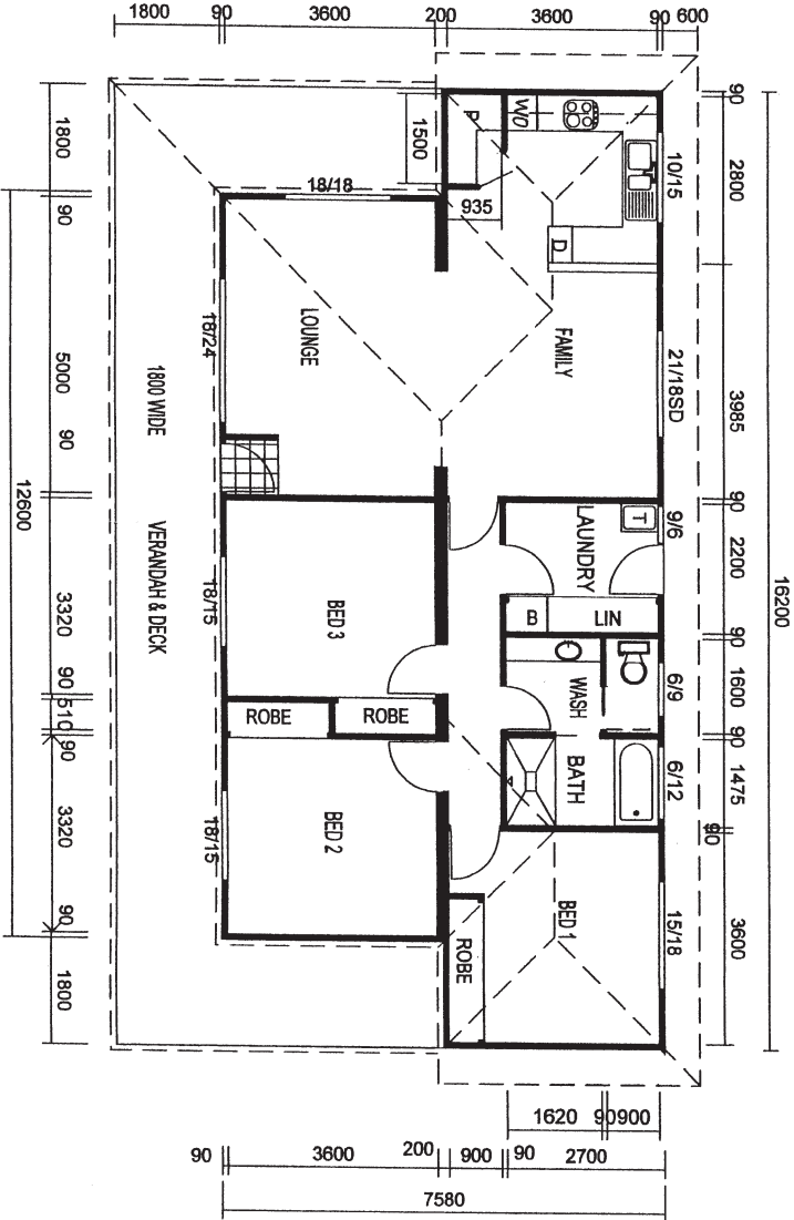
FLOOR PLAN
